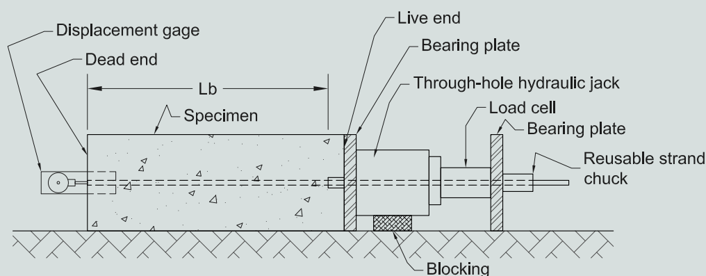
Figure 5.2.1.3. Strand block pullout test setup.
